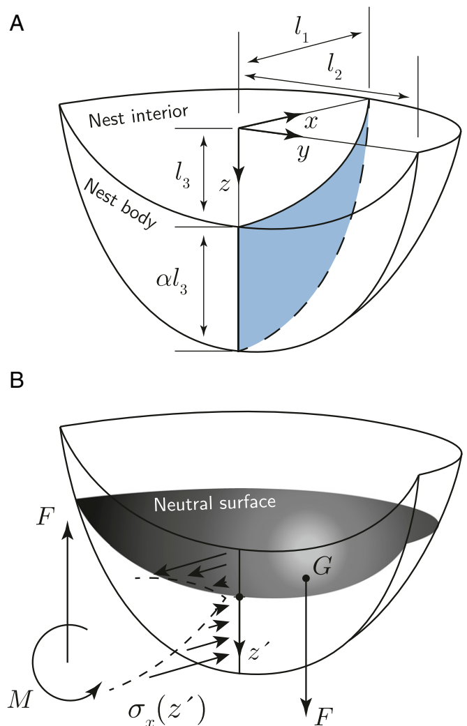
Fig. 4. Mud nest architecture. (A) Simplified geometry of half-cup-type mud nests. al_3 is defined as the vertical length of the nest body. (B) Free body diagram of an attached simplified mud nest. z' is the distance from the neutral surface at the adhered surface. G denotes a point of force application.
